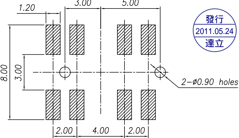
P.C.B Mounting pattern Dimension
