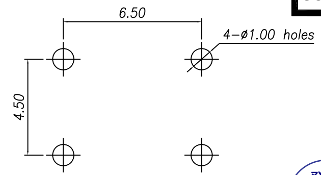
P.C.B Mounting pattern Dimension
