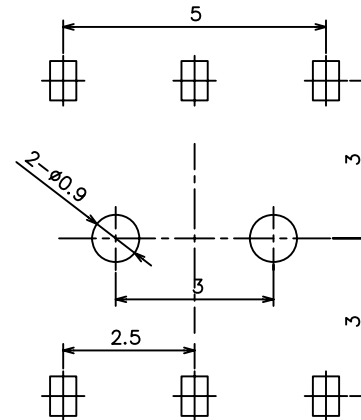
P.C.B Mounting pattern Dimension
