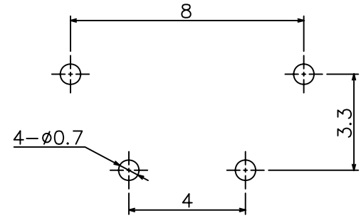
P.C.B Mounting pattern Dimension
