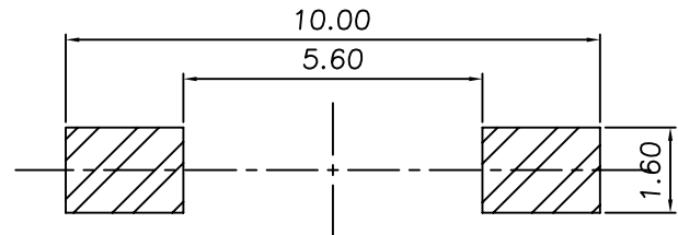
P.C.B Mounting pattern Dimension
