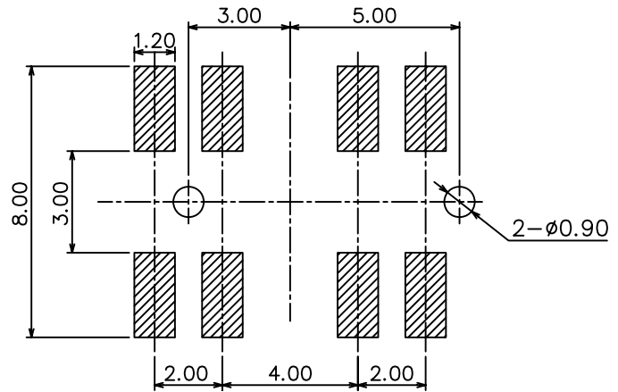
P.C.B Mounting pattern Dimension
