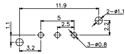
P.C.B Mounting pattern Dimension
