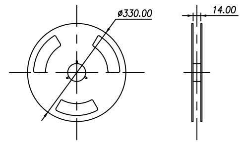
Carrier Taping Dimension
