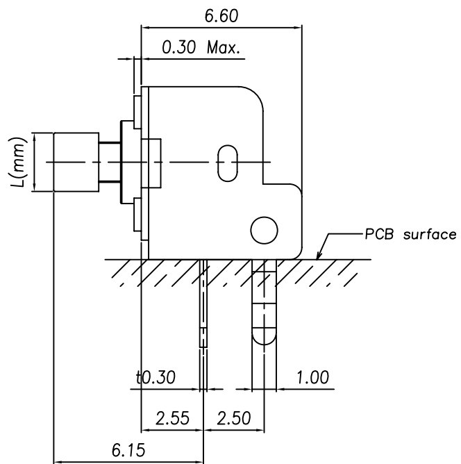
P.C.B Mounting pattern Dimension
