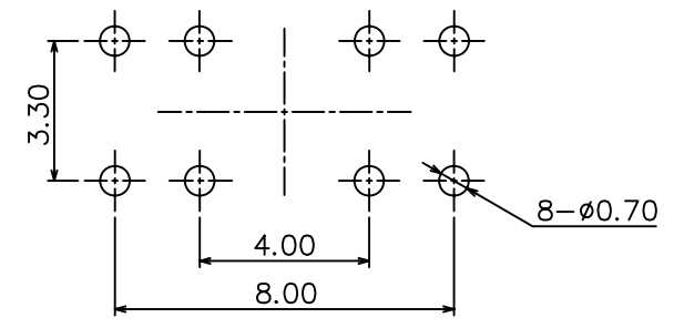
P.C.B Mounting pattern Dimension
