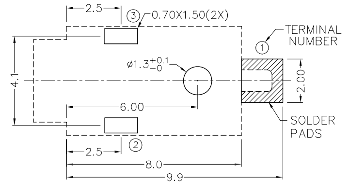
RECOMMENDED SOLDER PAD LAYOUT
