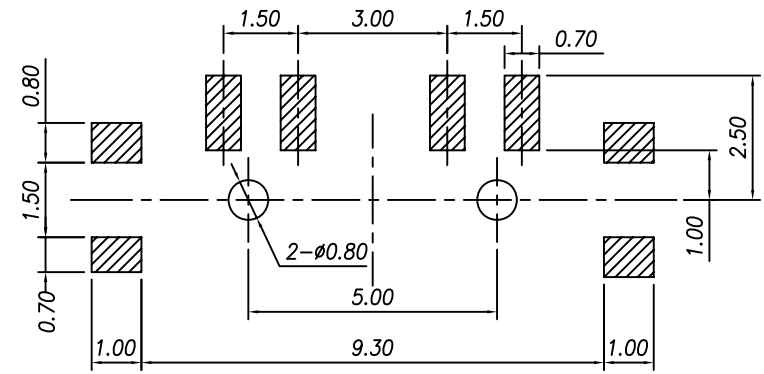
P.C.B Mounting pattern Dimension
