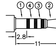
ø2.5 SPECIAL MATE PLUG
