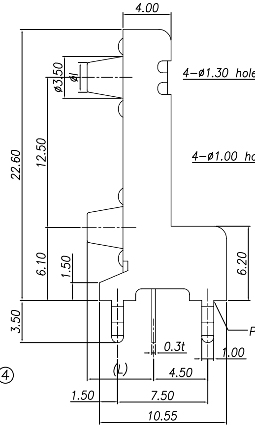
P.C.B Mounting pattern Dimension
