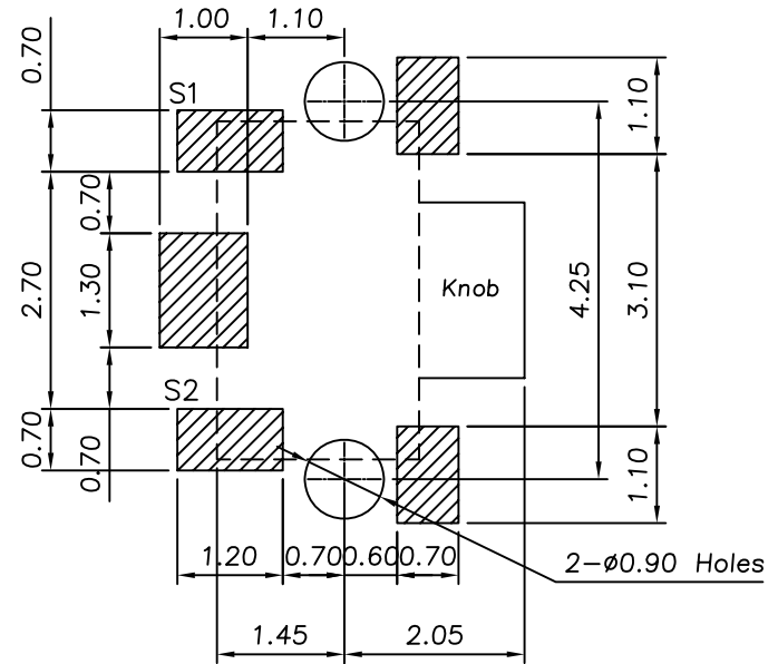
P.C.B Mounting pattern Dimension
