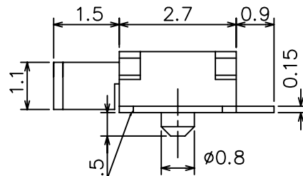
P.C BOARD MOUNTING FACE
