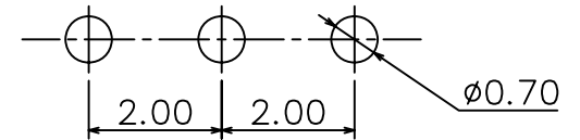
P.C.B Mounting pattern Dimension
